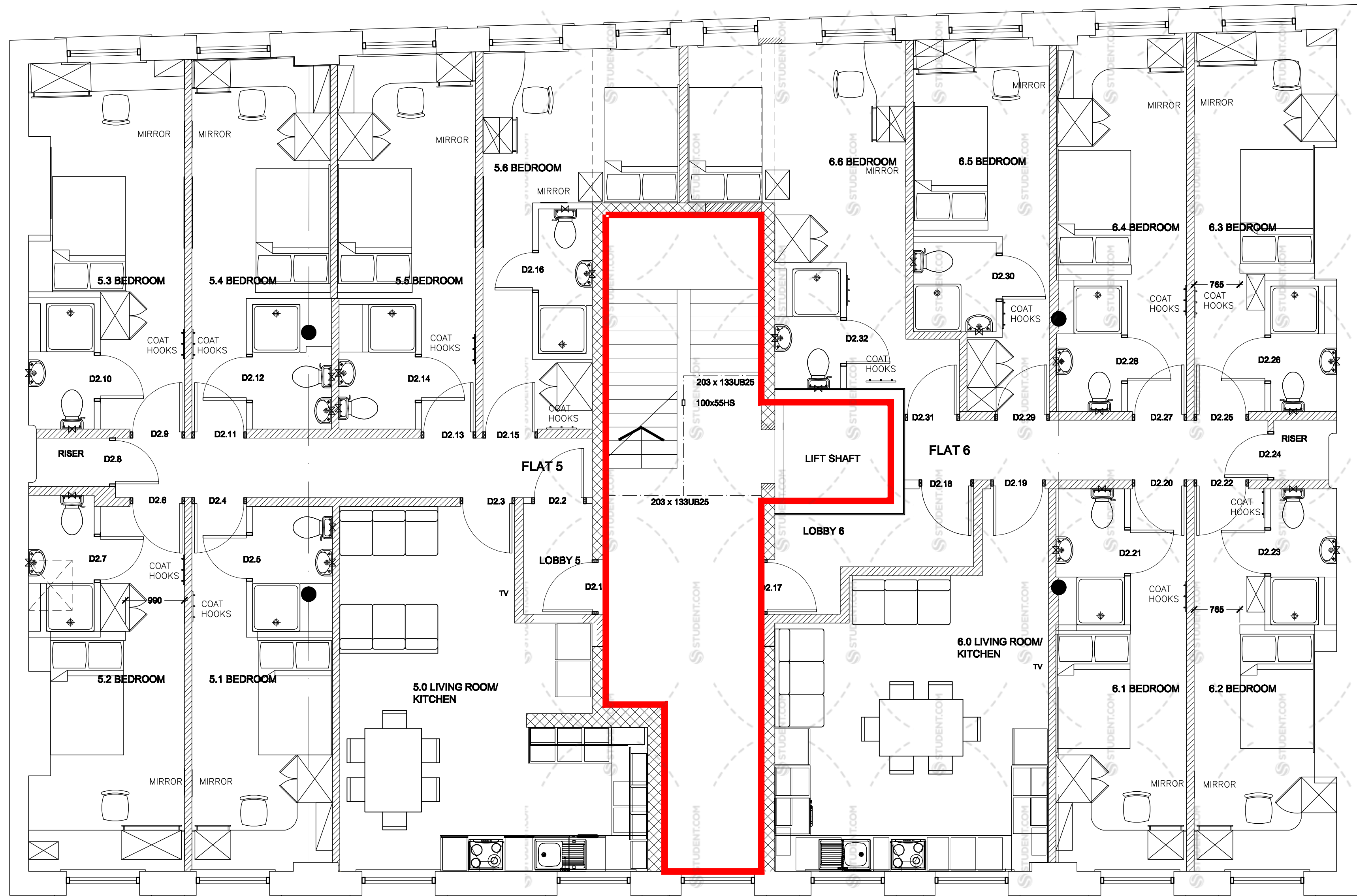
SECOND FLOOR
